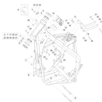
TAV.31 Telaio - Frame - Chassis - Rahmen - Chasis
